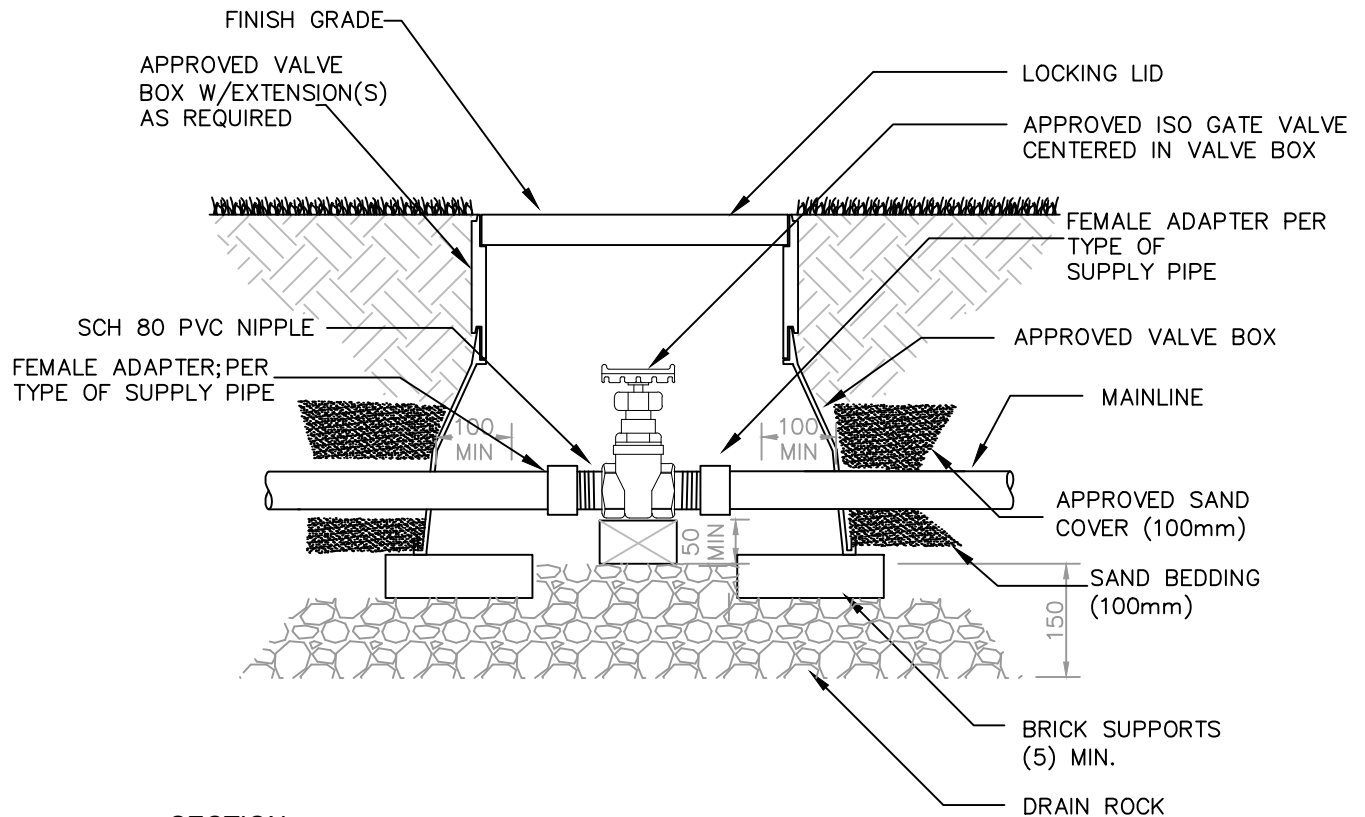
SECTION
