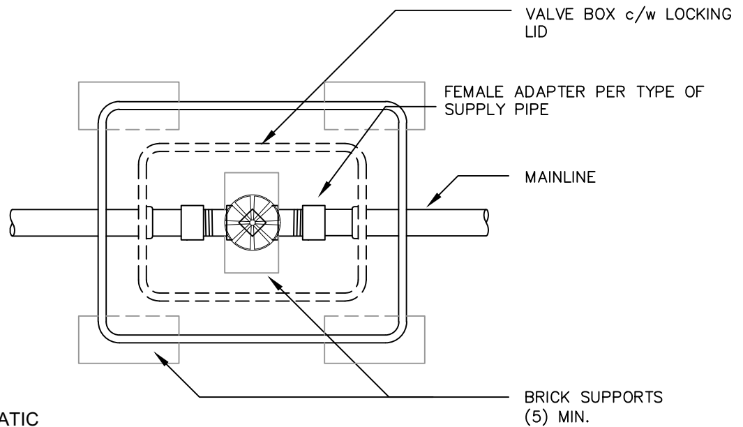
SCHEMATIC
