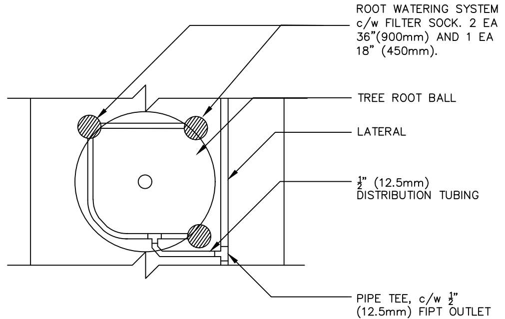
SCHEMATIC
