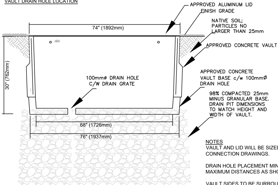
VAULT SECTION
